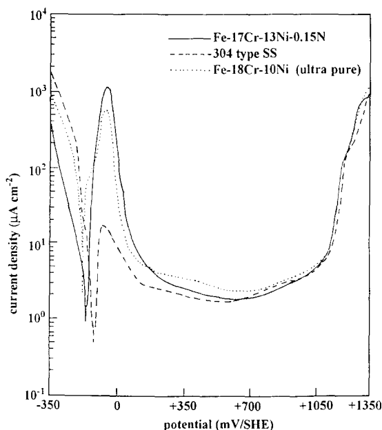
Fig. 1. Potentiodynamic curves for the three alloys in 0.5 M H_2SO_4 ( 1 \text{ mV s}^{-1} ).
