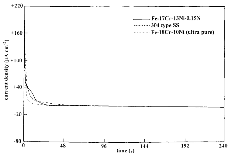
Fig. 2. Potentiostatic curves for the three alloys in 0.5 M H_2SO_4 (at 650 mV(SHE)).
